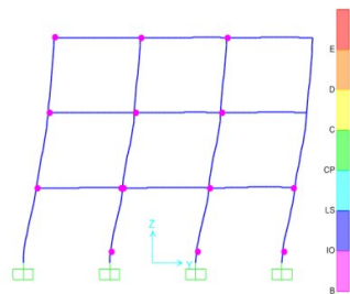
Fig. 13e Deformed Shape of the Frame-2 for Makkah (Y-Dir)
