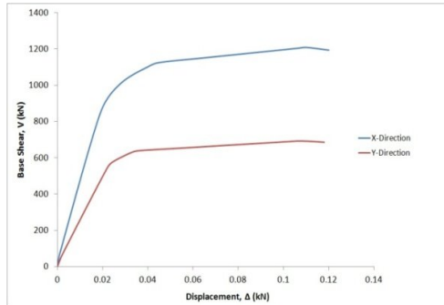
Fig. 7 Pushover Curve
