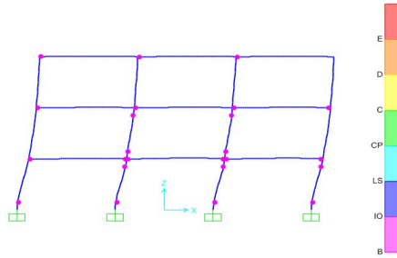
Fig. 11c Deformed Shape of the Frame-2 for Gizan (X-Dir)
