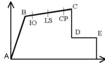
Fig. 3 Typical load-deformation relation and target performance level
