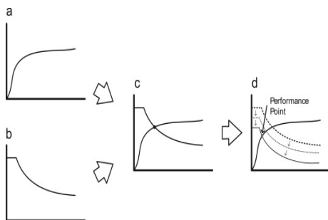
Fig. 2 Capacity Spectrum Method
