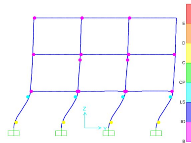
Fig. 16h Deformed Shape of the Frame-2 for Haql (Y-Dir)
