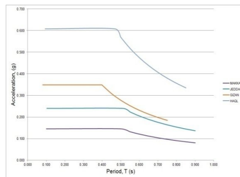
Fig. 6 Response Spectrum Curve for Each Region
