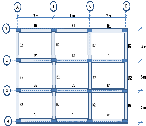
Fig. 4 Structural Layout
