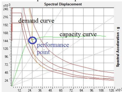
Fig. 8 Capacity Spectrum
